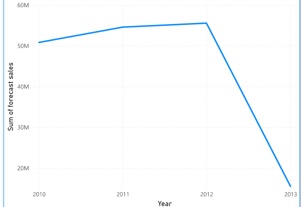
Forecast sales
